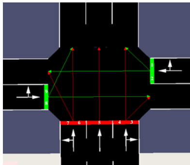
Fig. 12 Traffic signals at intersection 8
