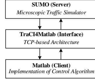
Fig. 18 Interactive simulation framework
