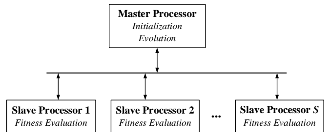
Fig. 19 Implementation of parallel fitness evaluation
