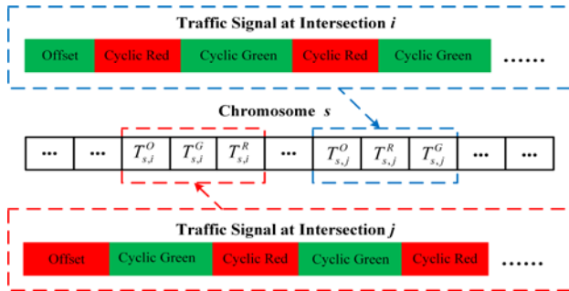
Fig. 5 Chromosome representation
